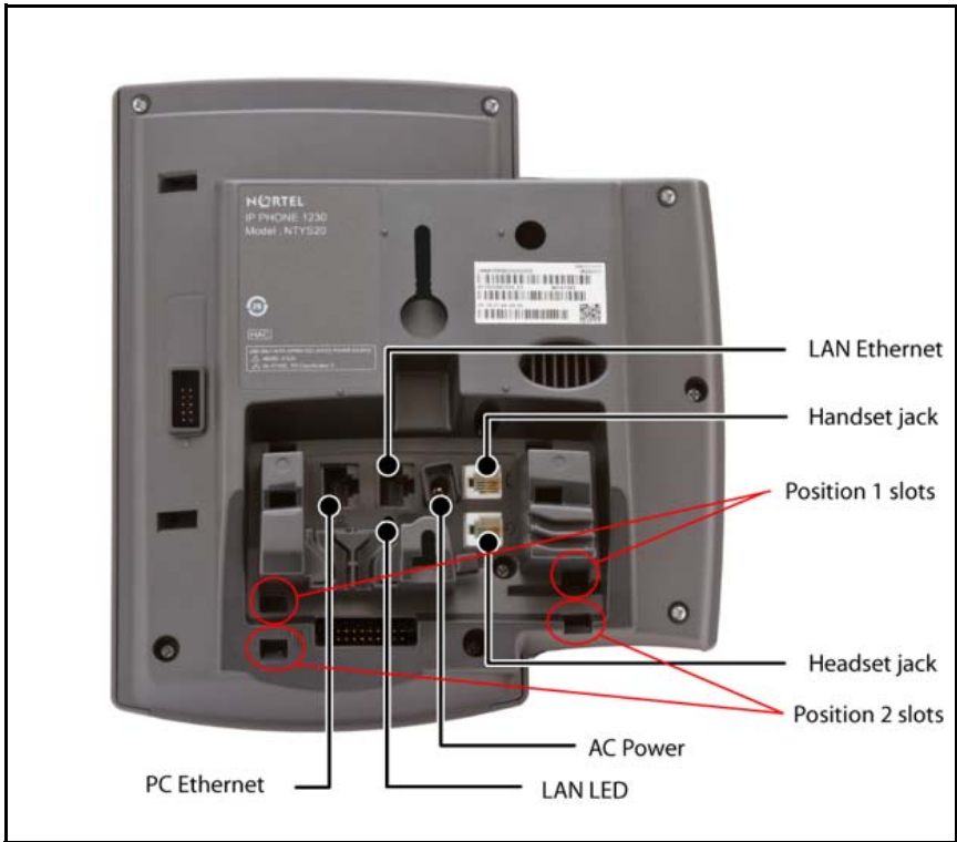
Figure 4: Connections on the IP Phone 1230
